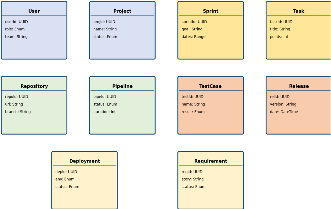
NeuroForge Nexus - Class Diagram: SDLC Domain
